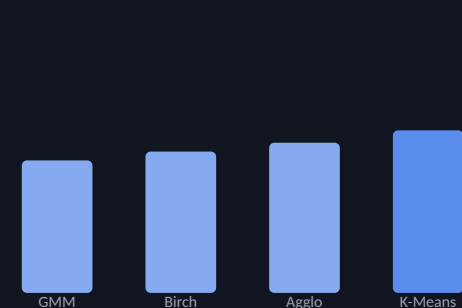
Silhouette Score
