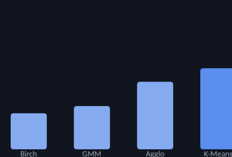
Calinski-Harabasz Score
